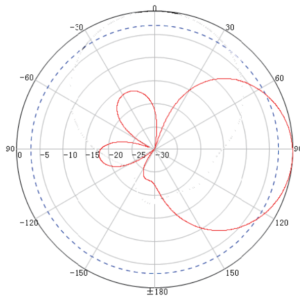
H Plane
