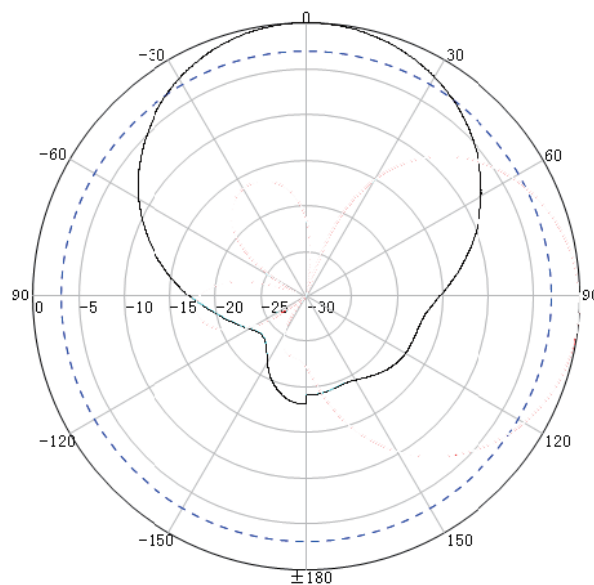
E Plane
