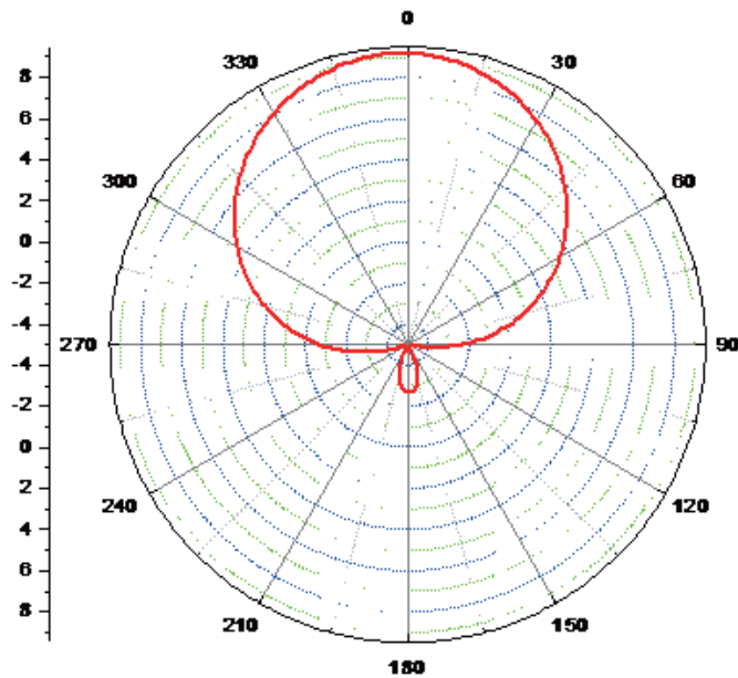
H Plane
