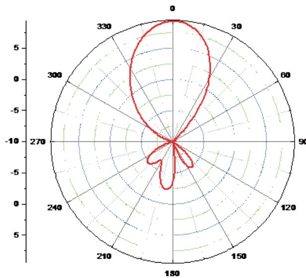
E Plane
