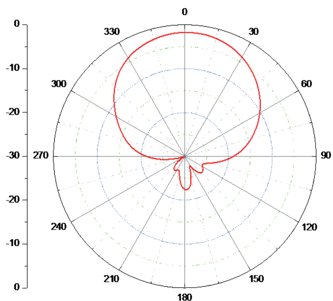
E Plane
